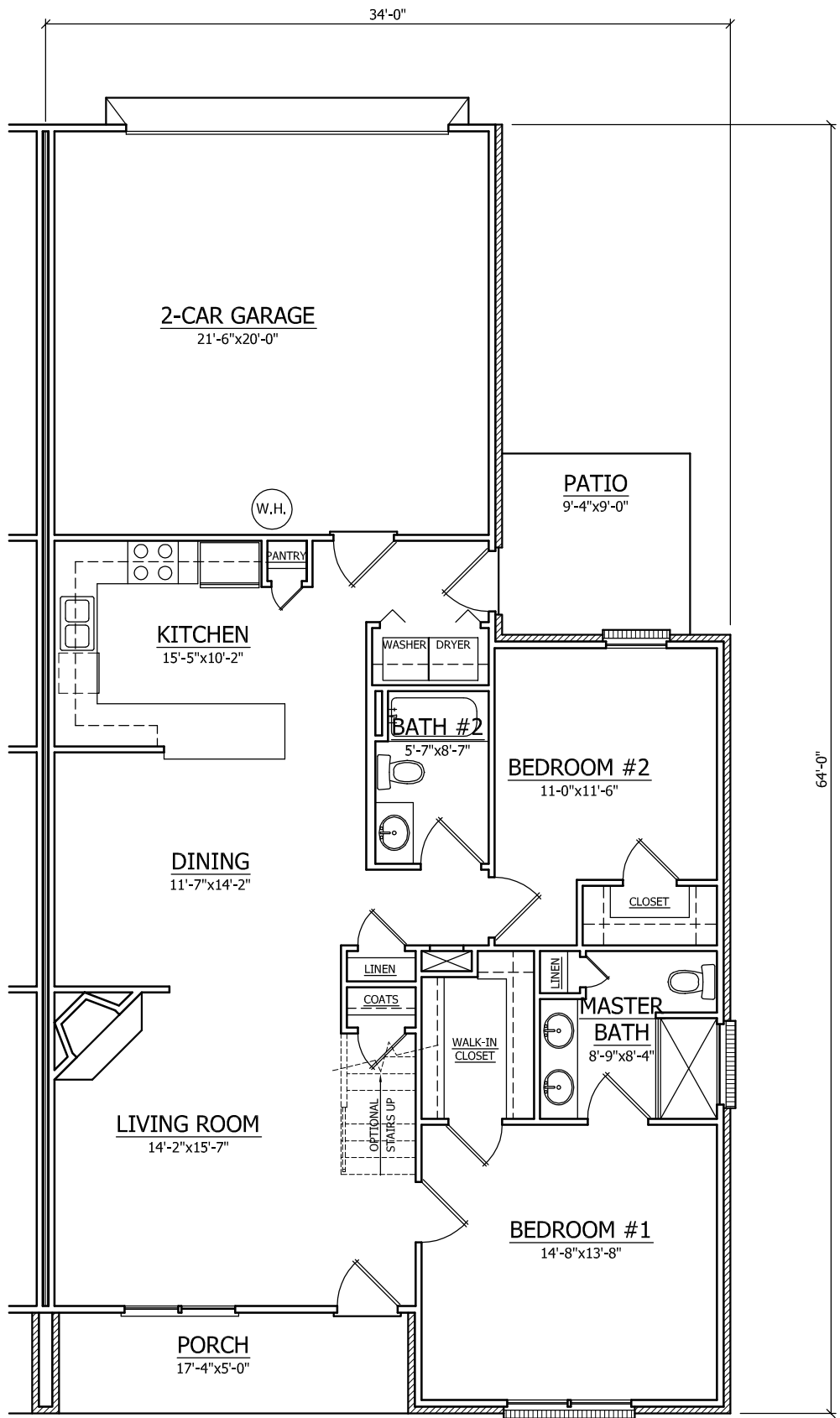
MAIN FLOOR PLAN 1/8" = 1'-0" ARCHITECTURAL DESIGNS SUBJECT TO CHANGE WITHOUT NOTICE
